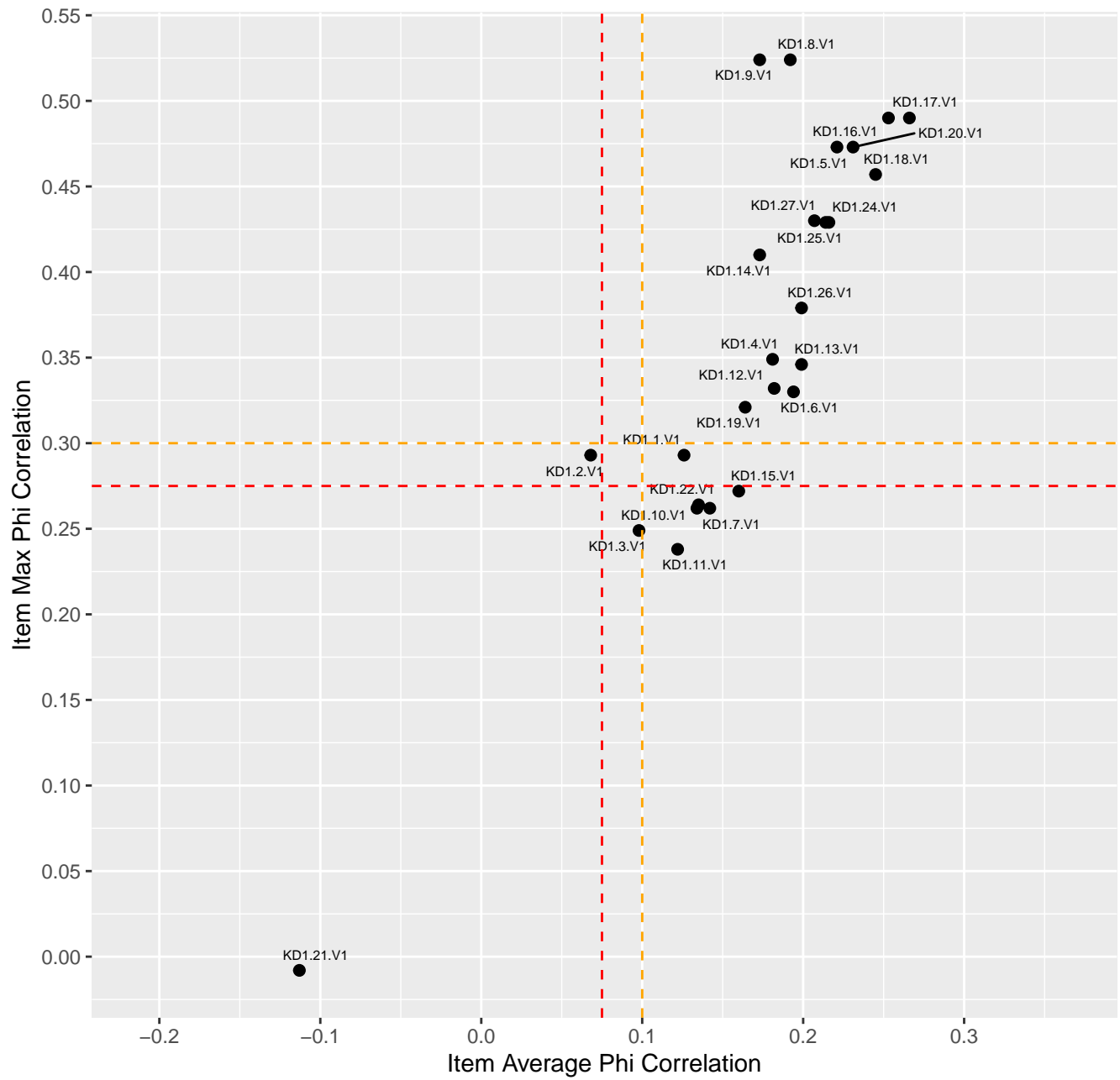
Item Average Phi Correlation vs Item Max Phi Correlation
