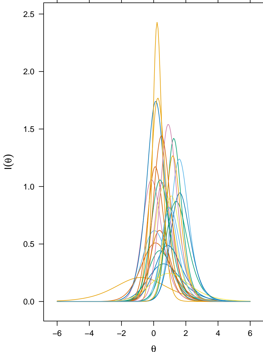
3PL IRT Model With All Items
