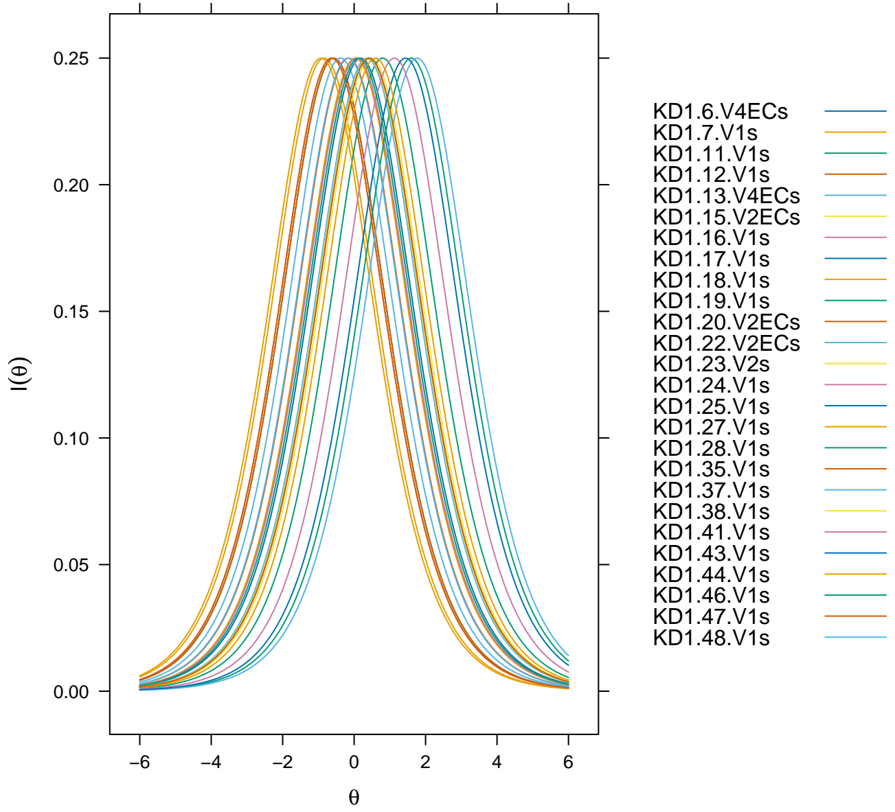
Rasch IRT Model With All Items
