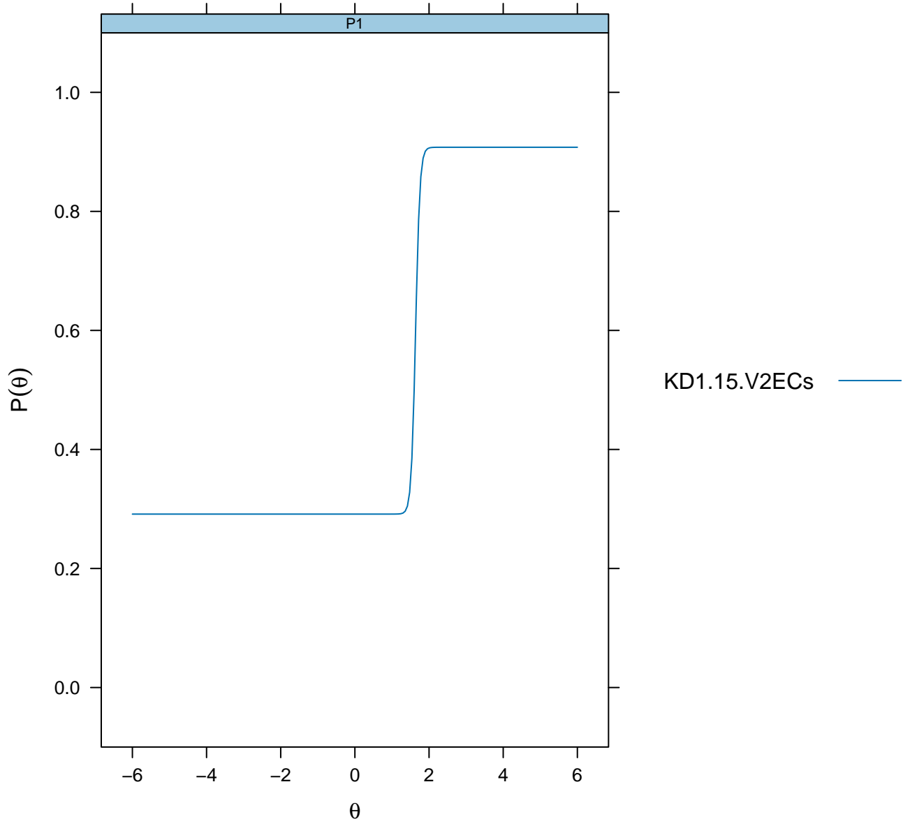
4PL IRT Model
