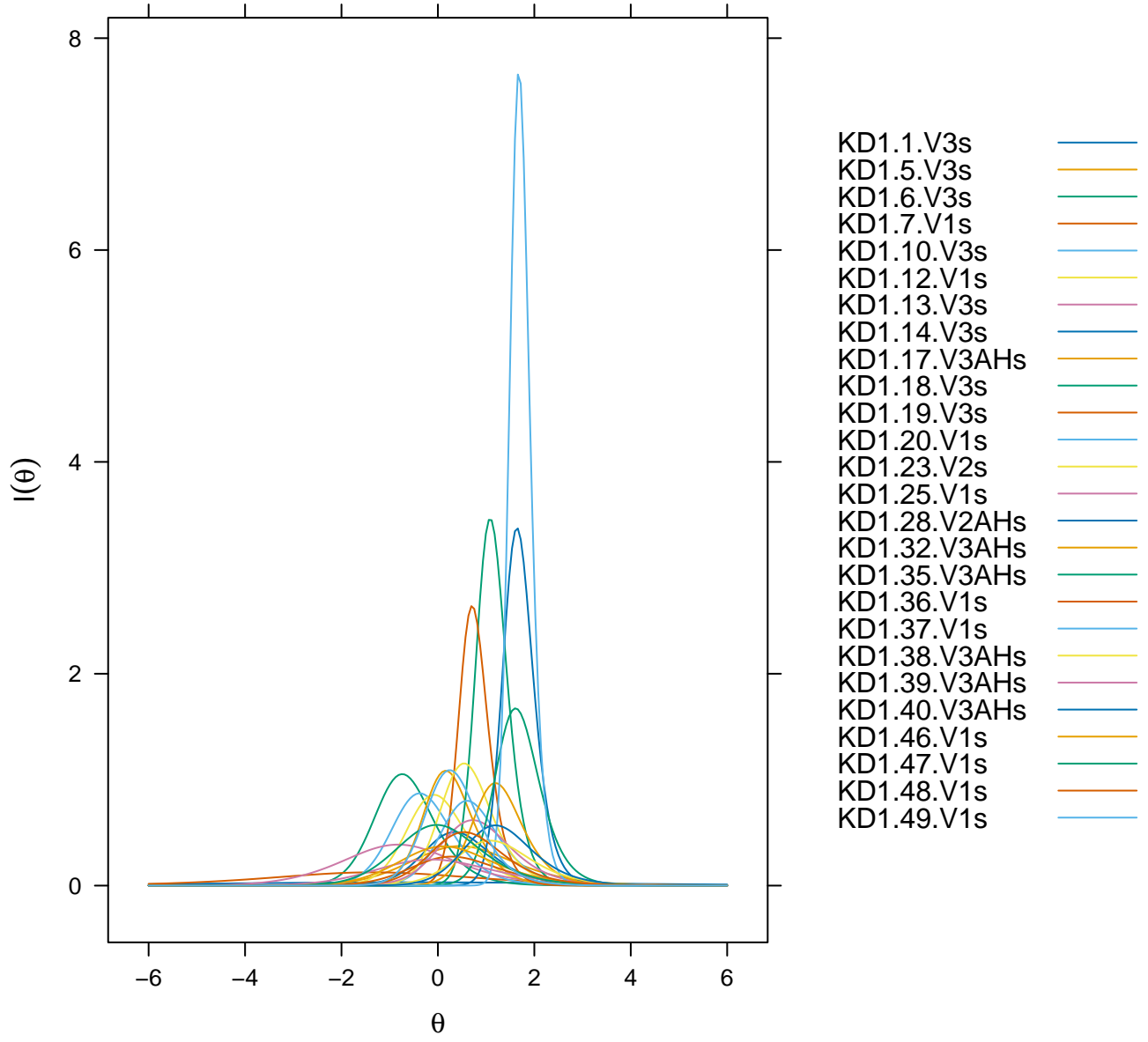
3PL IRT Model With All Items
