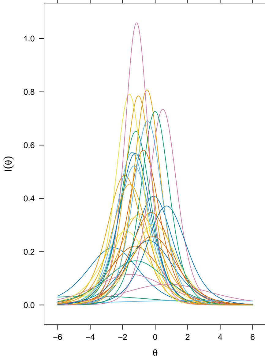
2PL IRT Model With All Items
