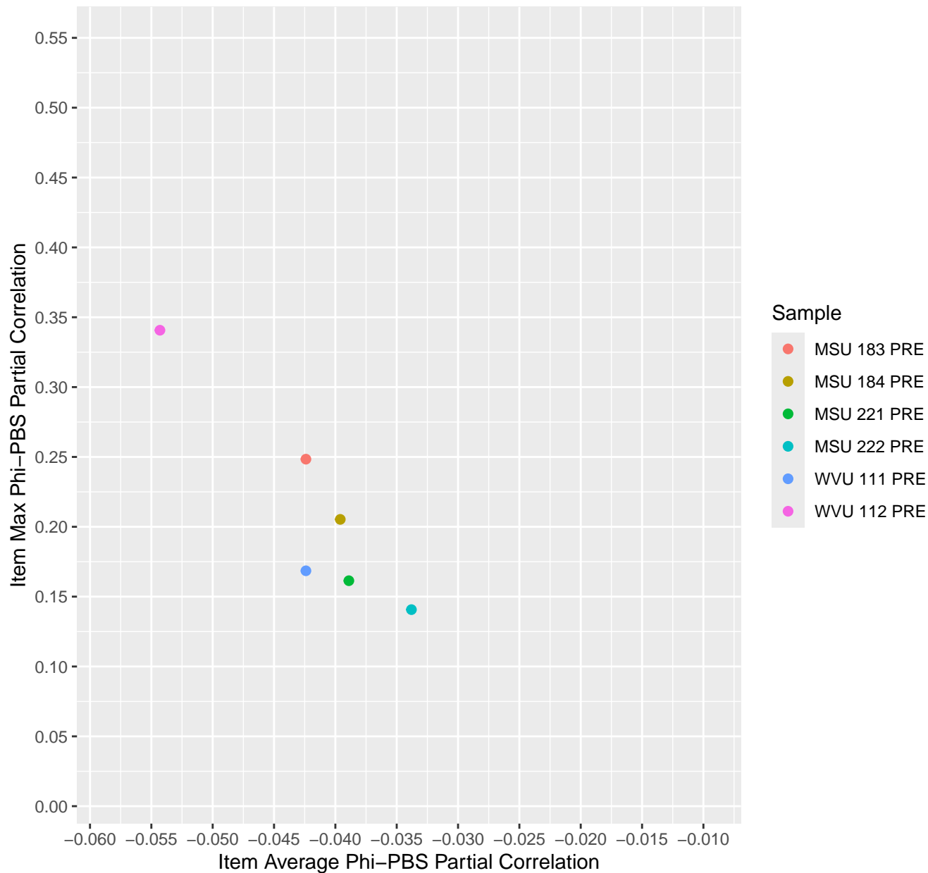
Item Average vs Max Phi-PBS Partial Correlation For KD1.5.V1
