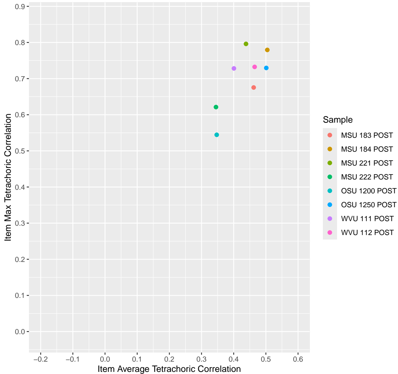
Item Average vs Max Tetrachoric Correlation For KD1.47.V1
