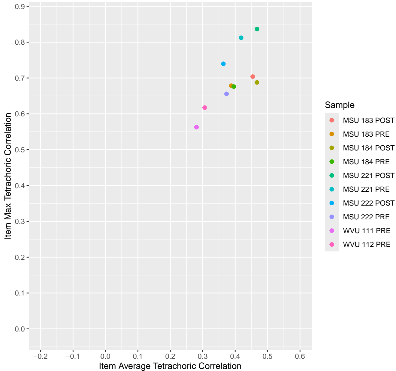
Item Average vs Max Tetrachoric Correlation For KD1.18.V1
