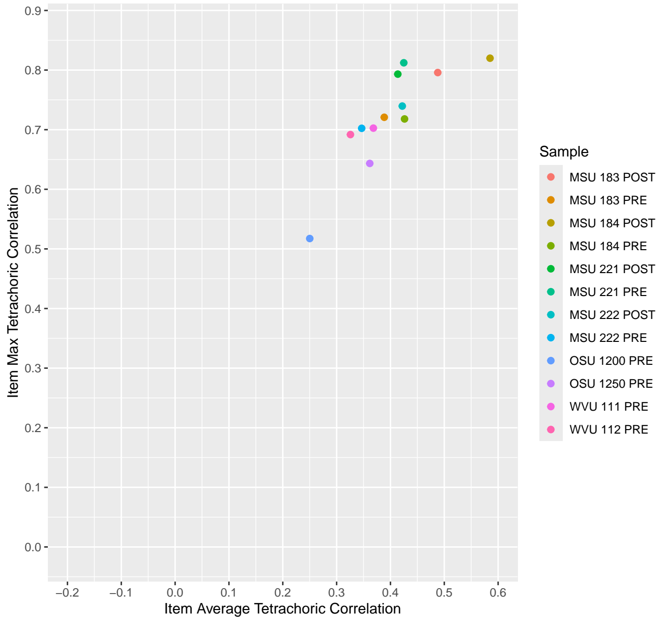
Item Average vs Max Tetrachoric Correlation For KD1.17.V1
