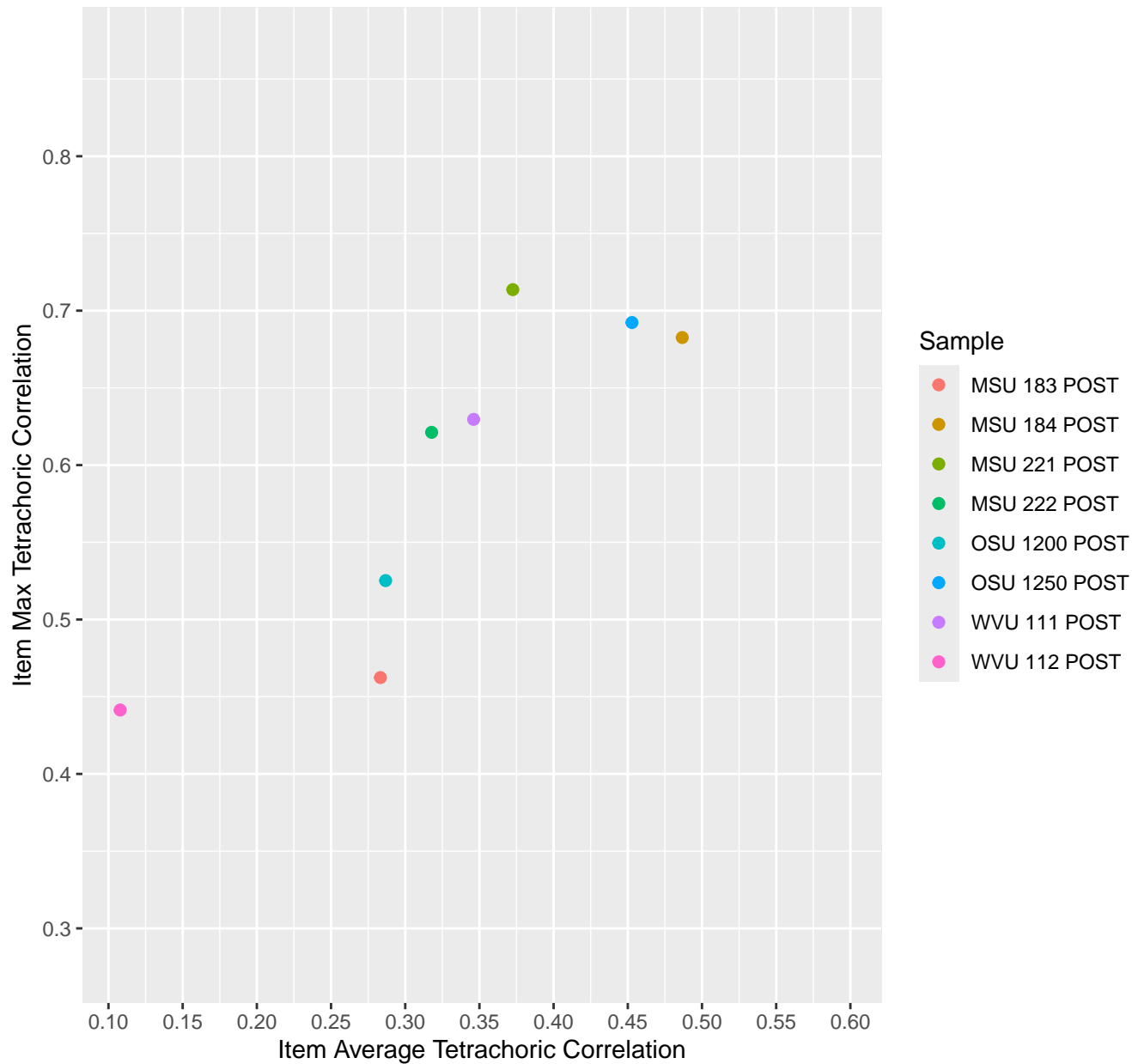
Item Average vs Max Tetrachoric Correlation For KD1.48.V1
