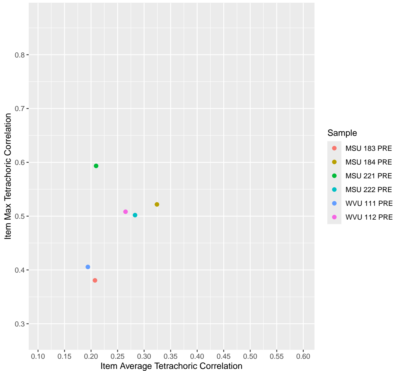
Item Average vs Max Tetrachoric Correlation For KD1.13.V1
