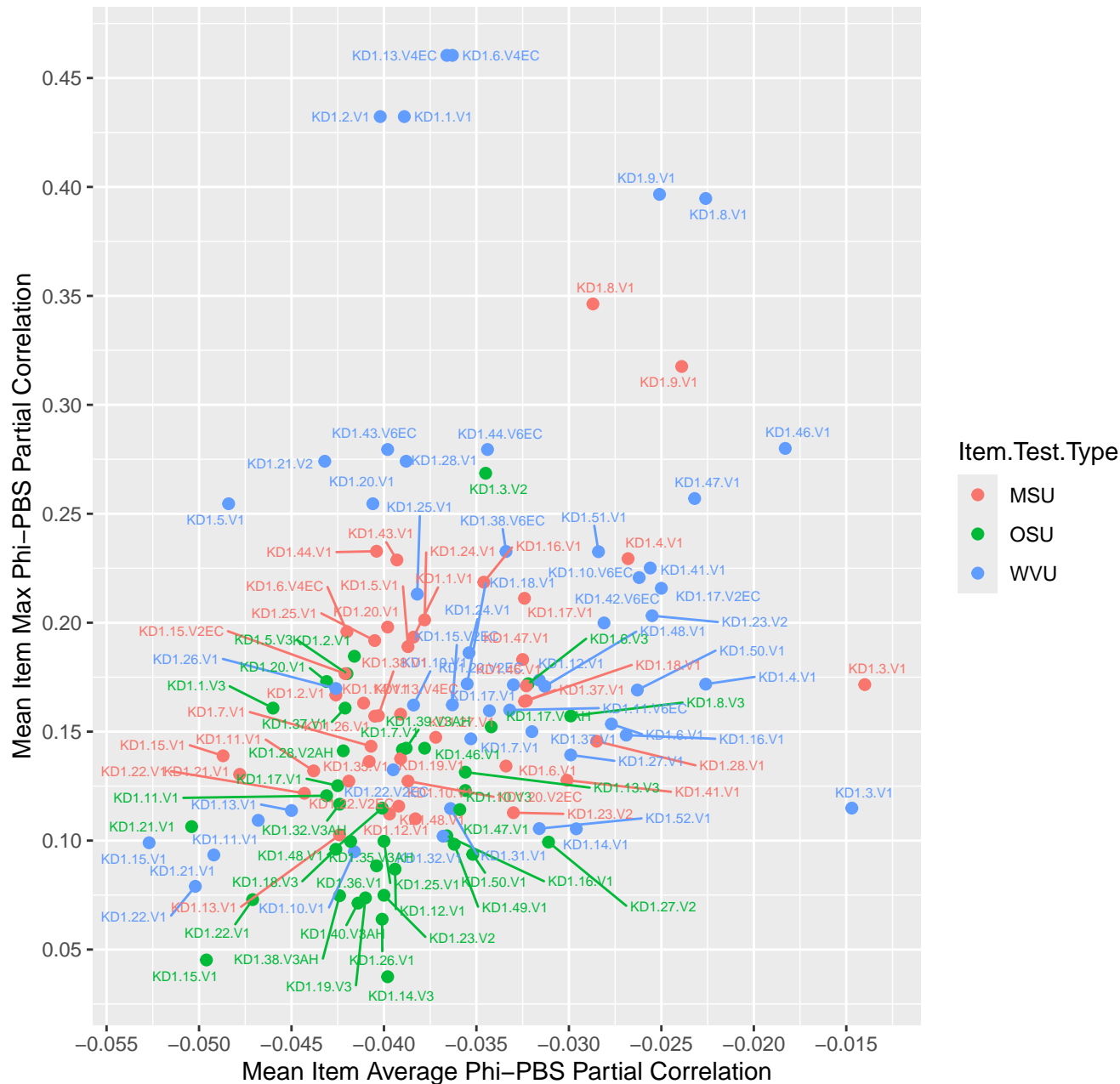
Mean Item Average vs Max Phi-PBS Partial Correlation
