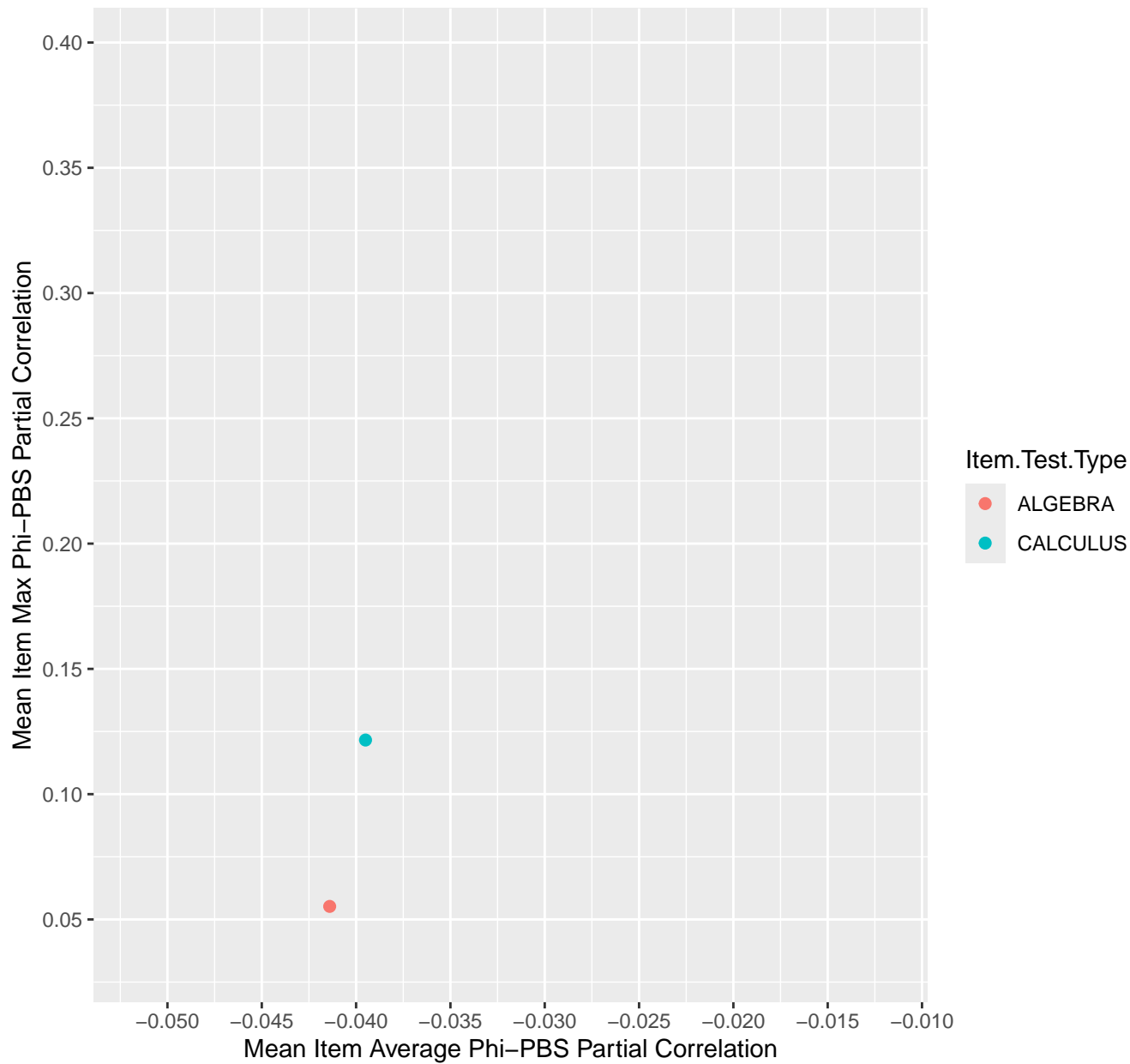
Mean Item Average vs Max Phi-PBS Partial Correlation For KD1.36.V1
