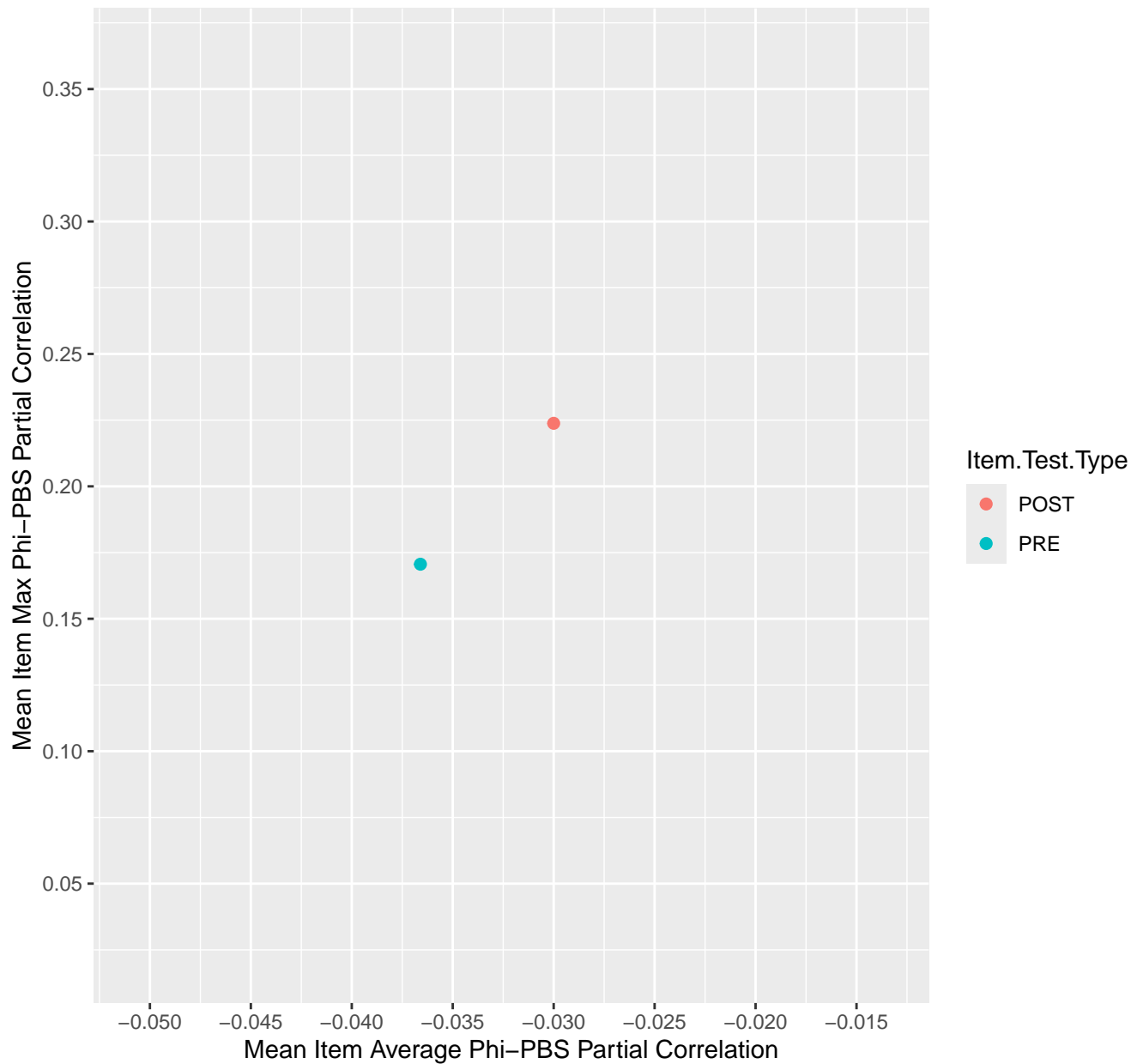
Mean Item Average vs Max Phi-PBS Partial Correlation For KD1.17.V1
