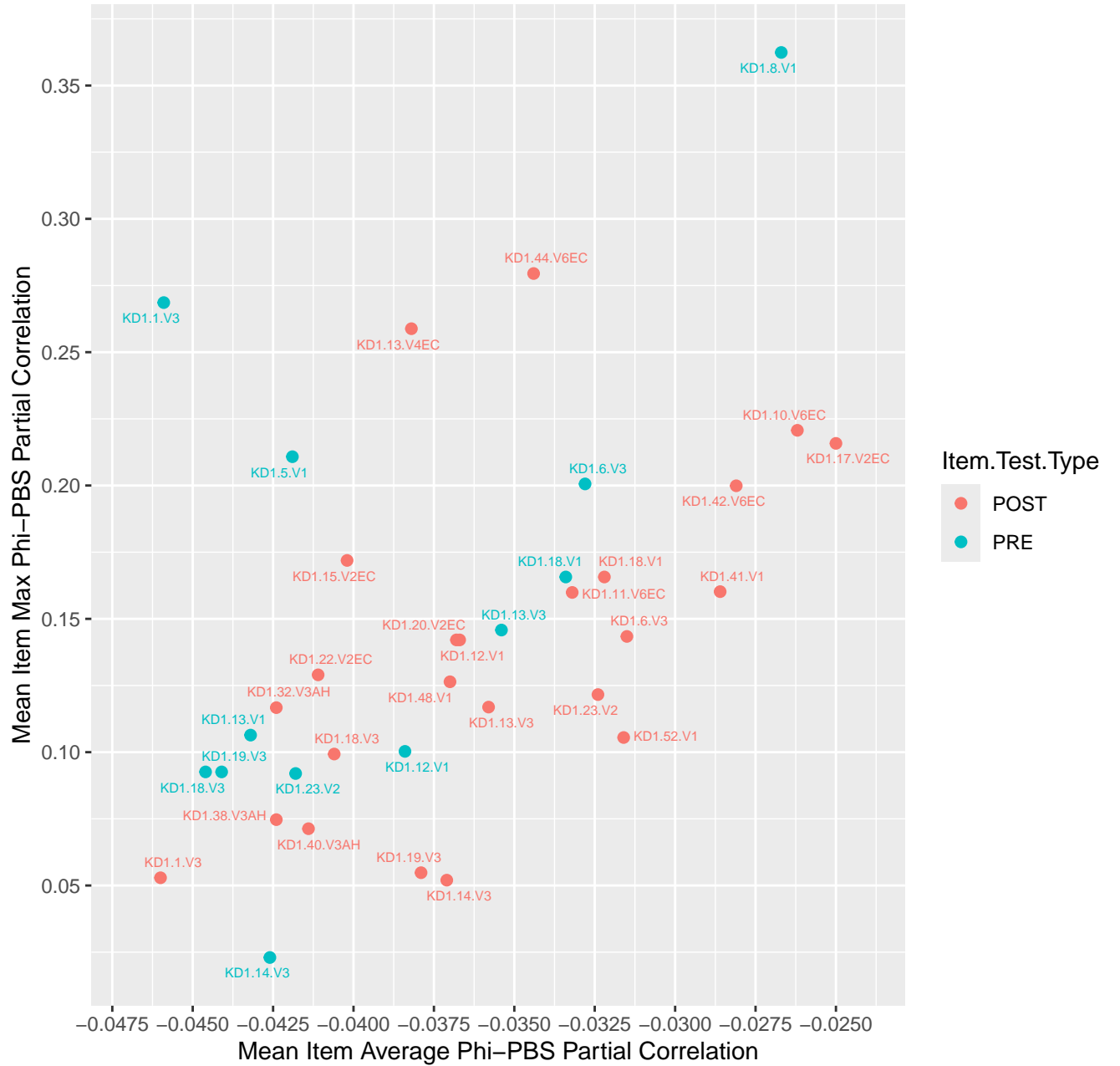
Mean Item Average Phi-PBS Partial Correlation vs Mean Item Max Phi-PBS Pa
