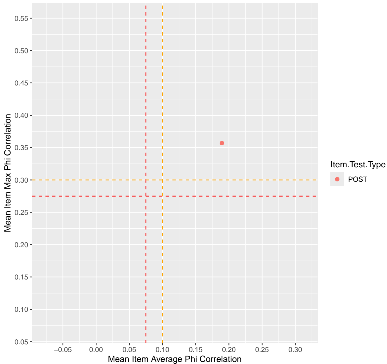
Mean Item Average vs Max Phi Correlation For KD1.11.V6EC
