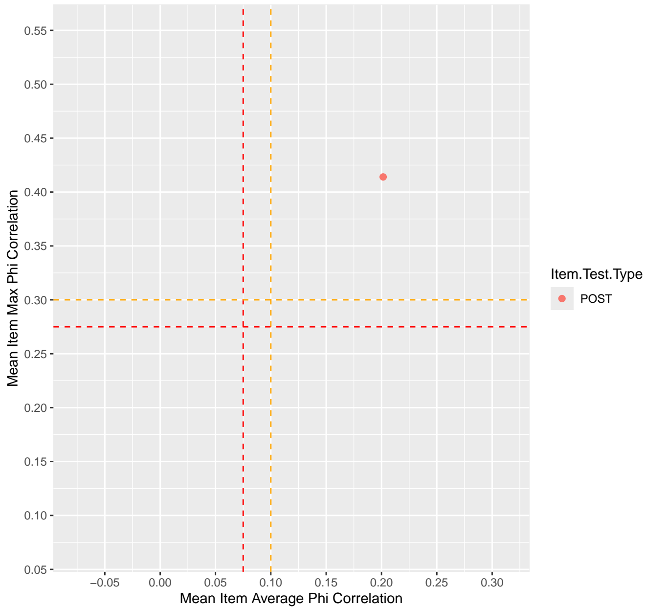
Mean Item Average vs Max Phi Correlation For KD1.17.V2EC
