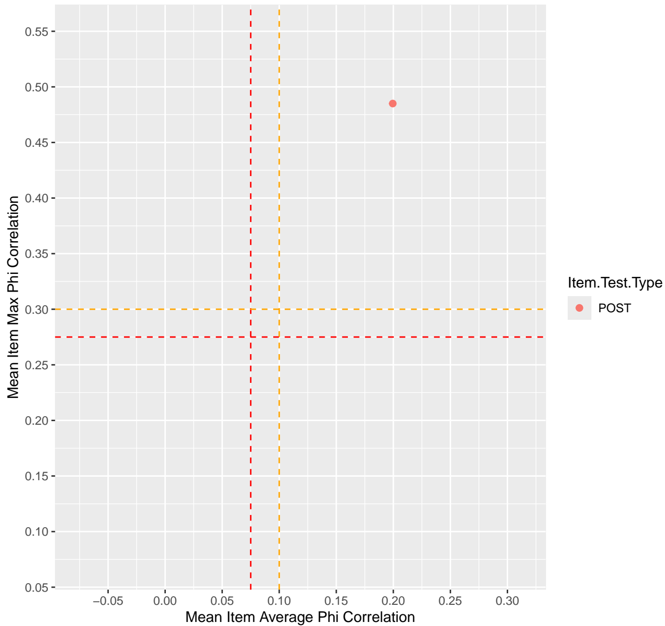
Mean Item Average vs Max Phi Correlation For KD1.43.V6EC
