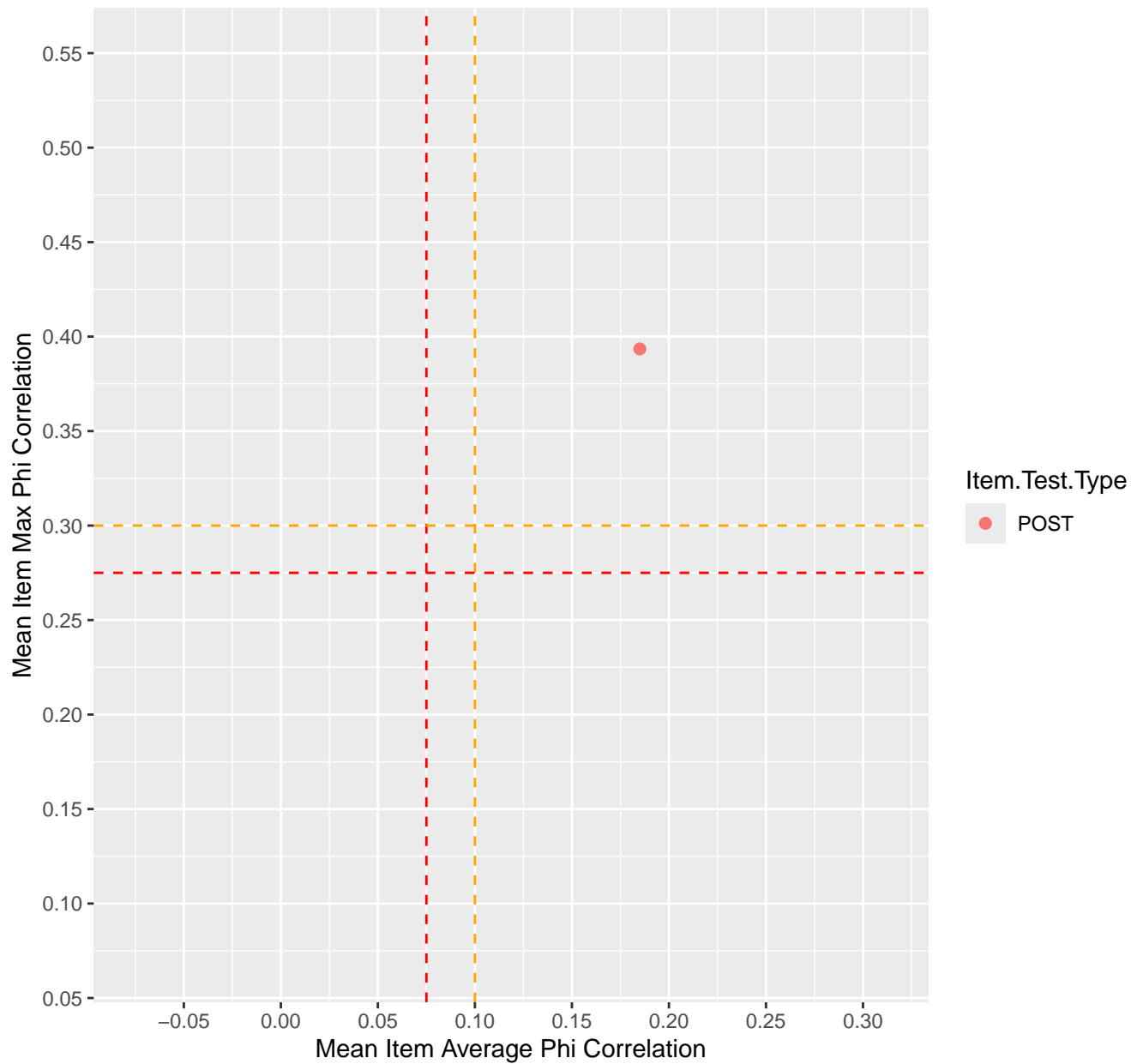
Mean Item Average vs Max Phi Correlation For KD1.10.V6EC
