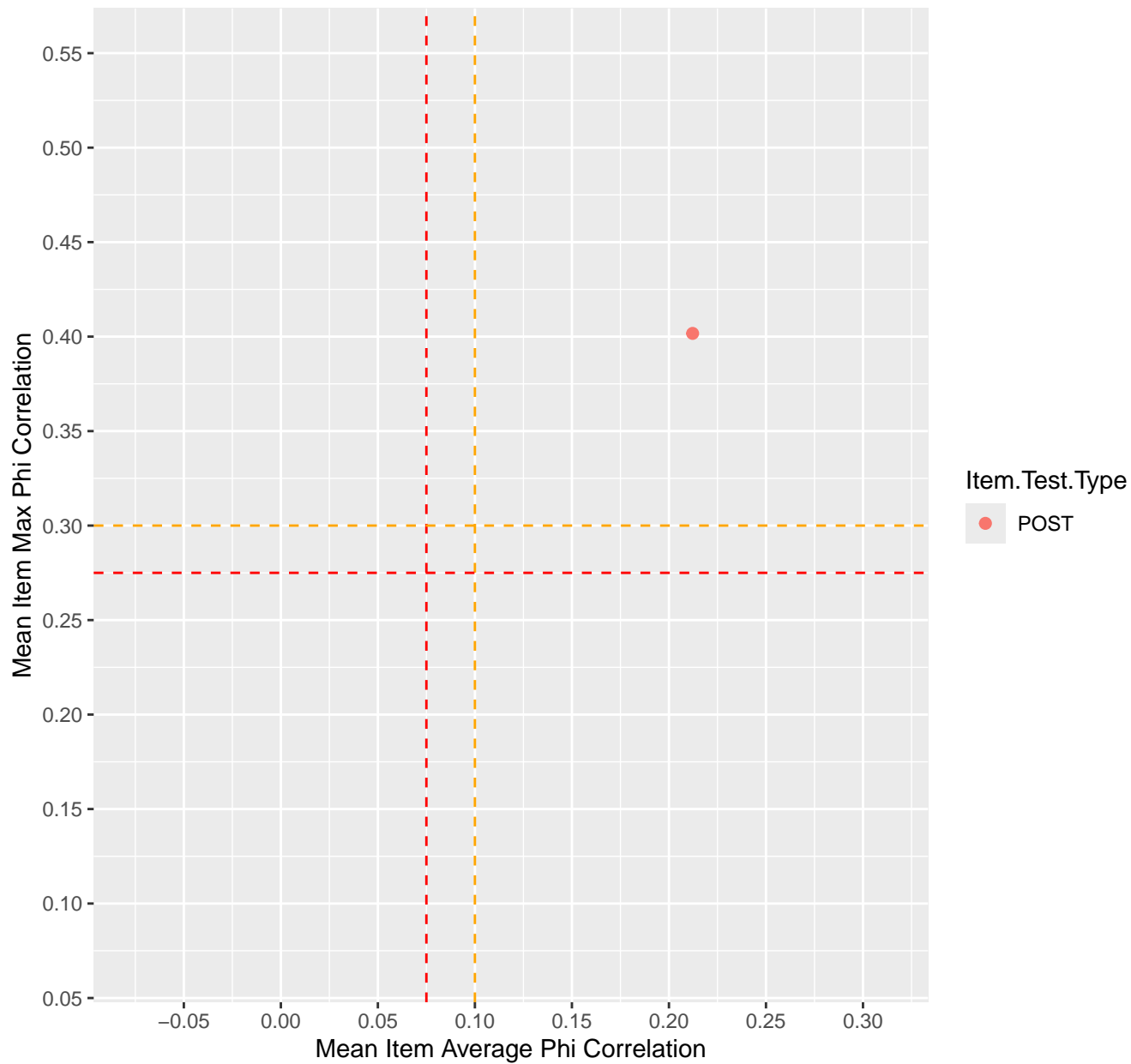
Mean Item Average vs Max Phi Correlation For KD1.20.V2EC
