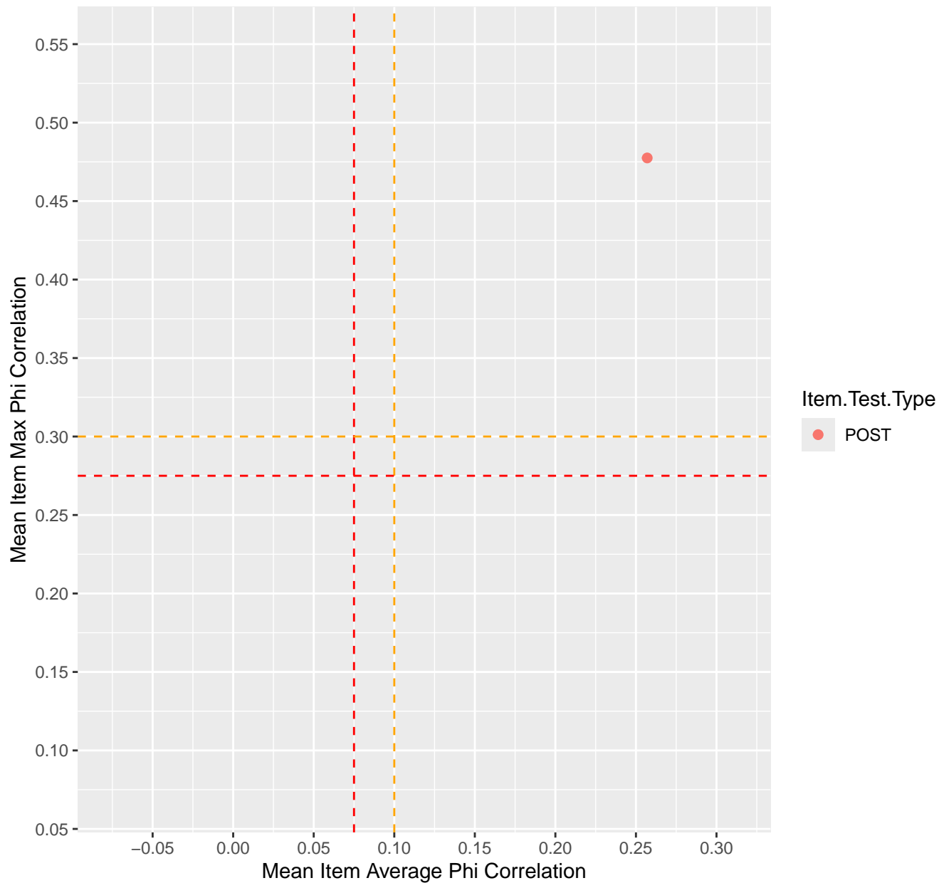
Mean Item Average vs Max Phi Correlation For KD1.42.V6EC
