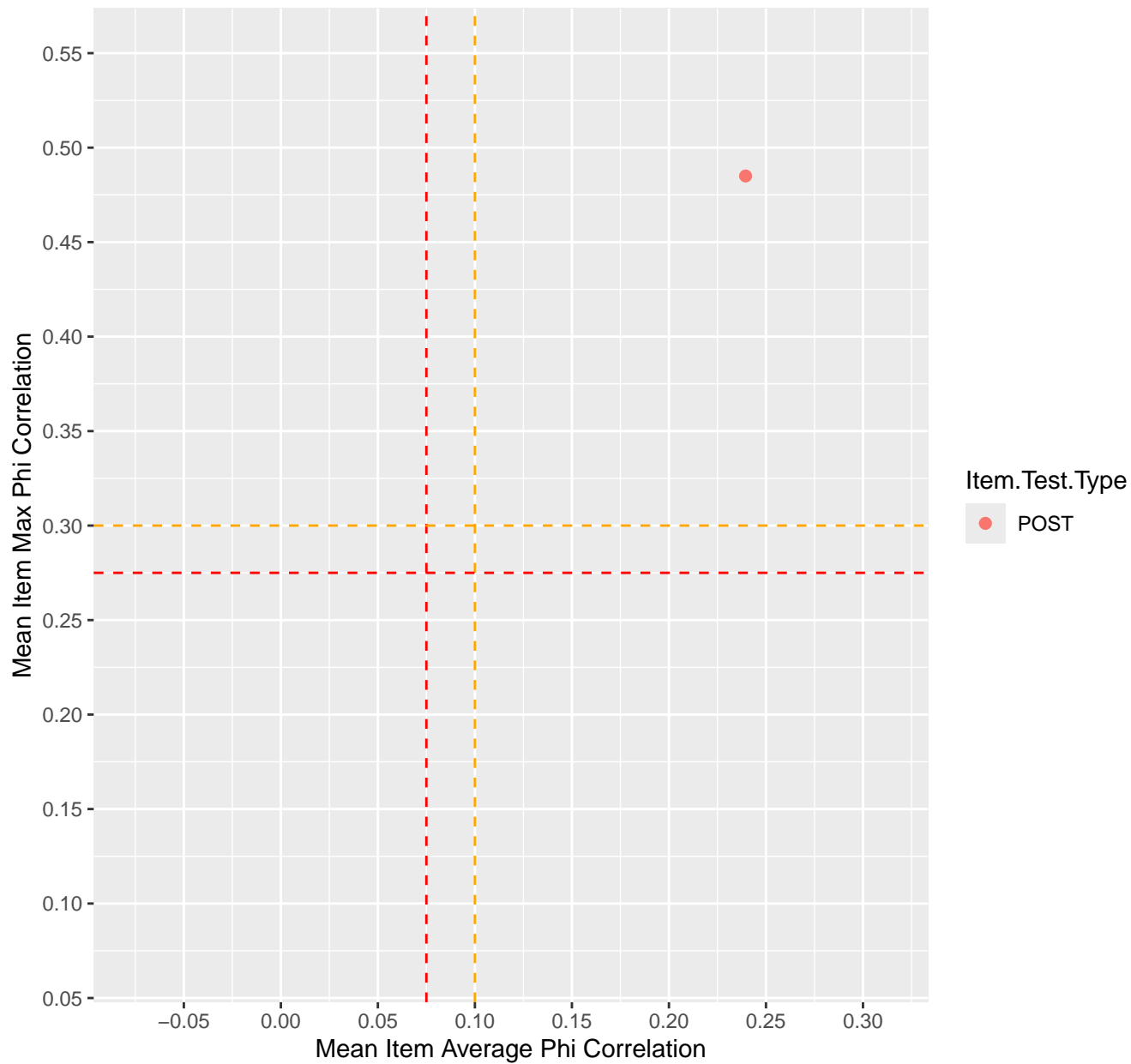
Mean Item Average vs Max Phi Correlation For KD1.44.V6EC
