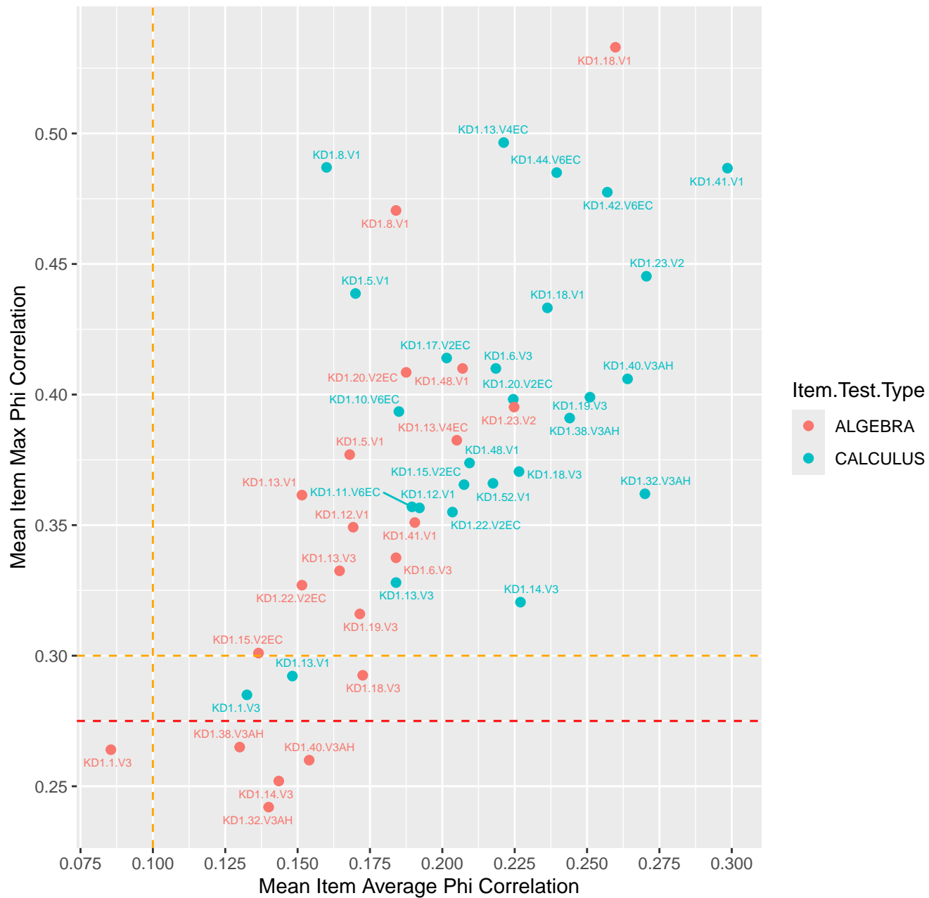
Mean Item Average vs Max Phi Correlation
