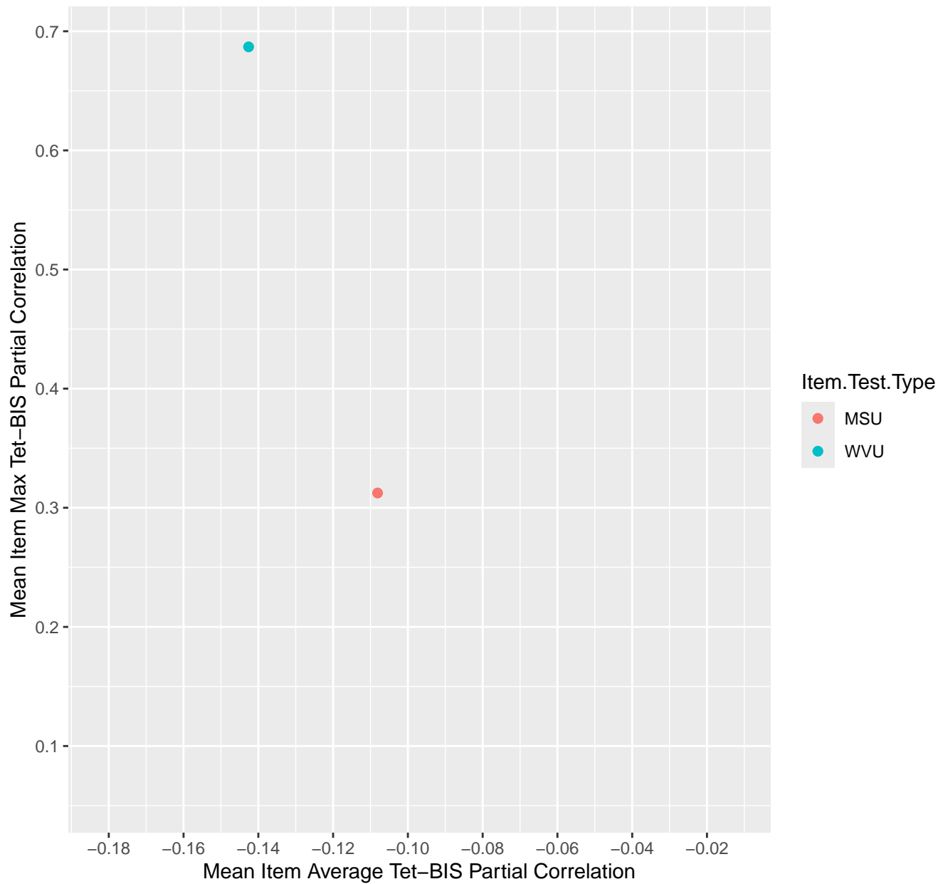
Mean Item Average vs Max Tet-BIS Partial Correlation For KD1.6.V4EC
