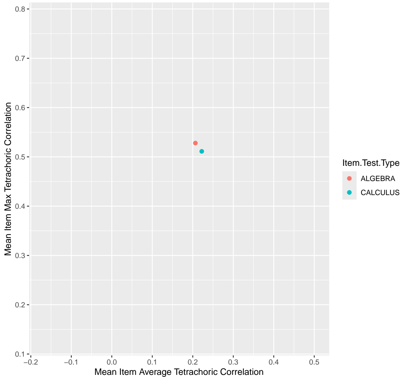
Mean Item Average vs Max Tetrachoric Correlation For KD1.26.V1
