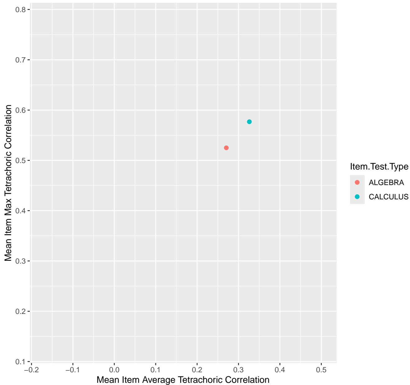
Mean Item Average vs Max Tetrachoric Correlation For KD1.12.V1
