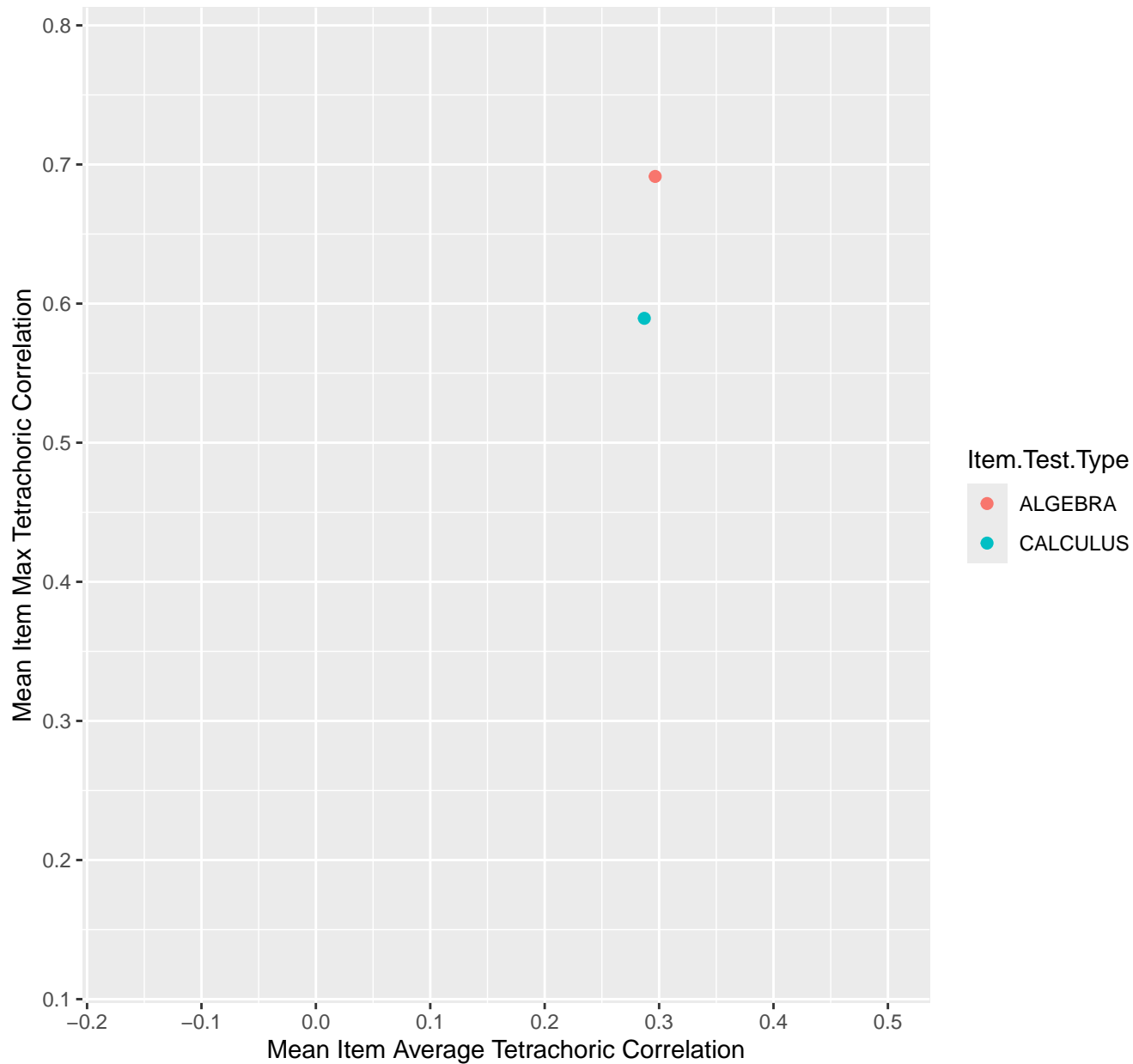
Mean Item Average vs Max Tetrachoric Correlation For KD1.6.V1
