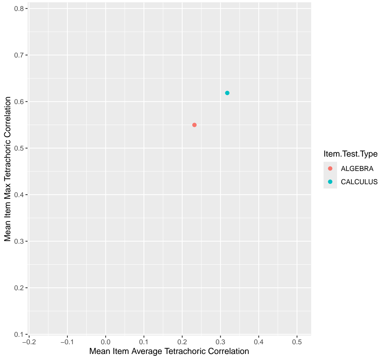
Mean Item Average vs Max Tetrachoric Correlation For KD1.27.V1
