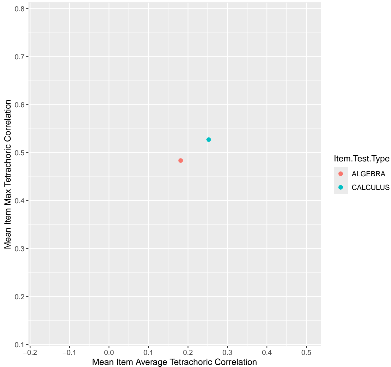
Mean Item Average vs Max Tetrachoric Correlation For KD1.50.V1
