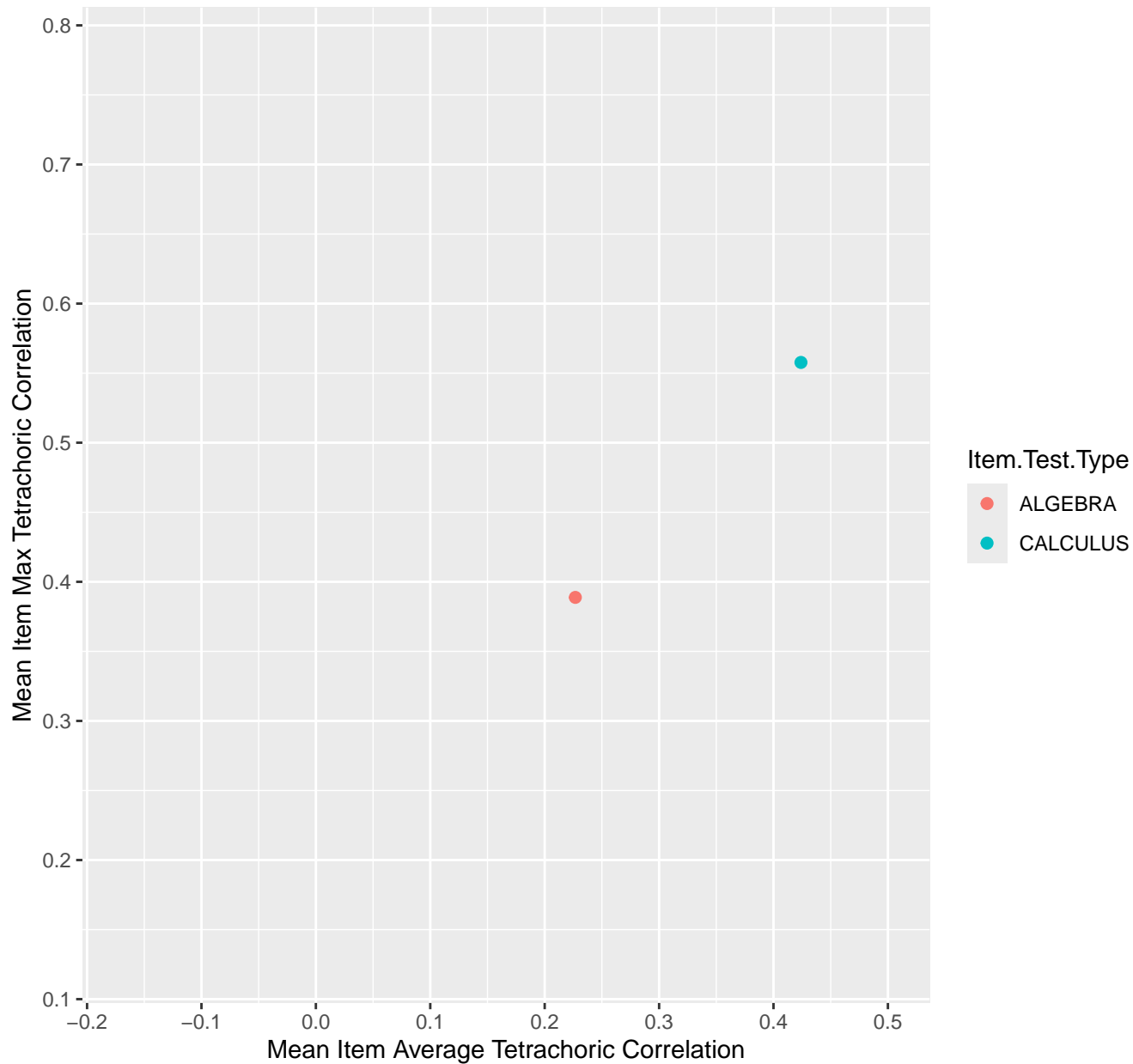
Mean Item Average vs Max Tetrachoric Correlation For KD1.32.V3AH
