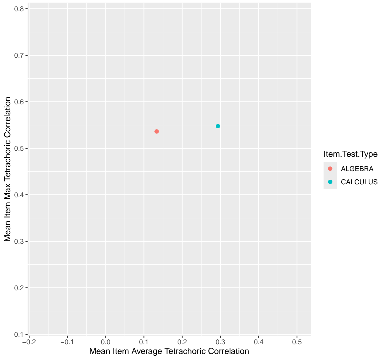
Mean Item Average vs Max Tetrachoric Correlation For KD1.43.V1
