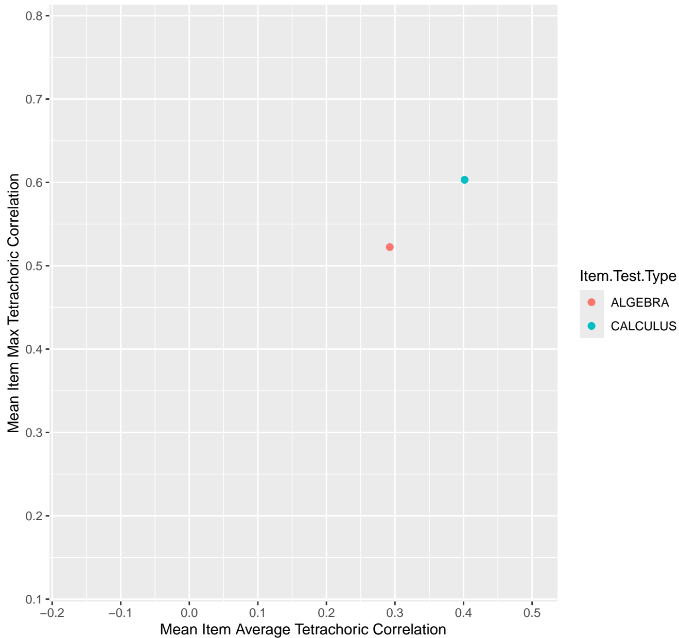
Mean Item Average vs Max Tetrachoric Correlation For KD1.10.V3
