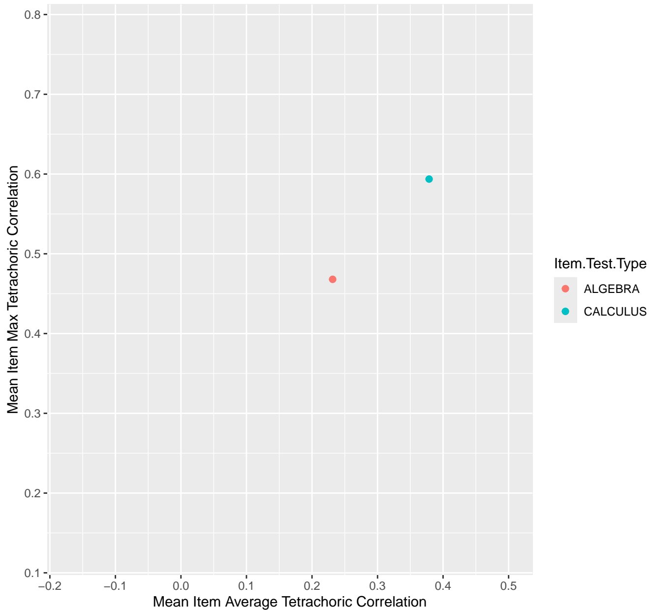
Mean Item Average vs Max Tetrachoric Correlation For KD1.27.V2
