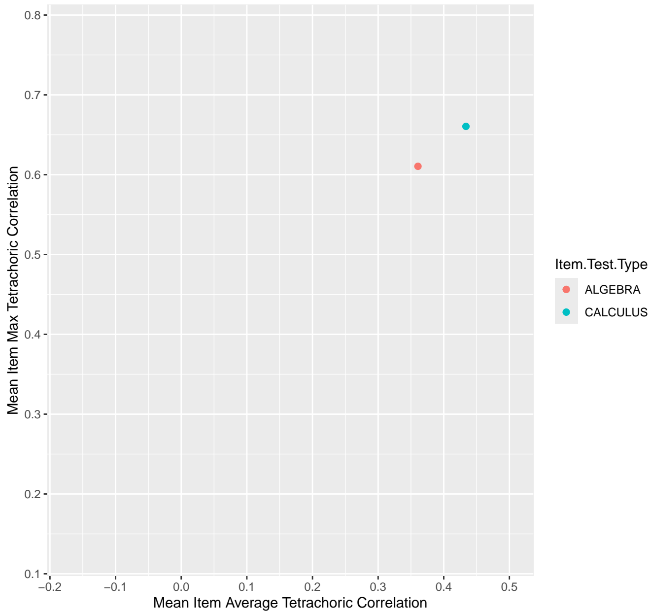
Mean Item Average vs Max Tetrachoric Correlation For KD1.23.V2
