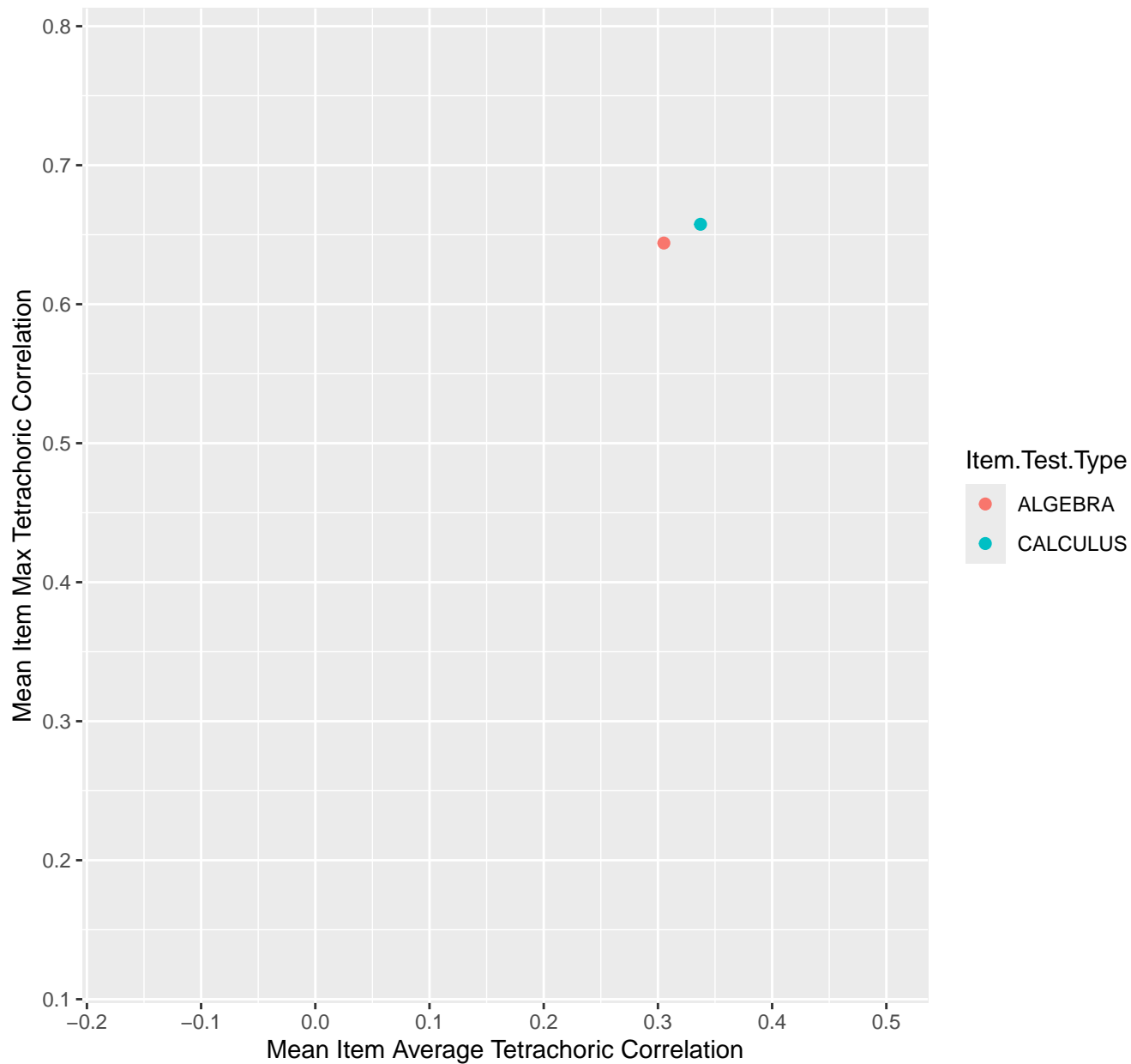
Mean Item Average vs Max Tetrachoric Correlation For KD1.24.V1
