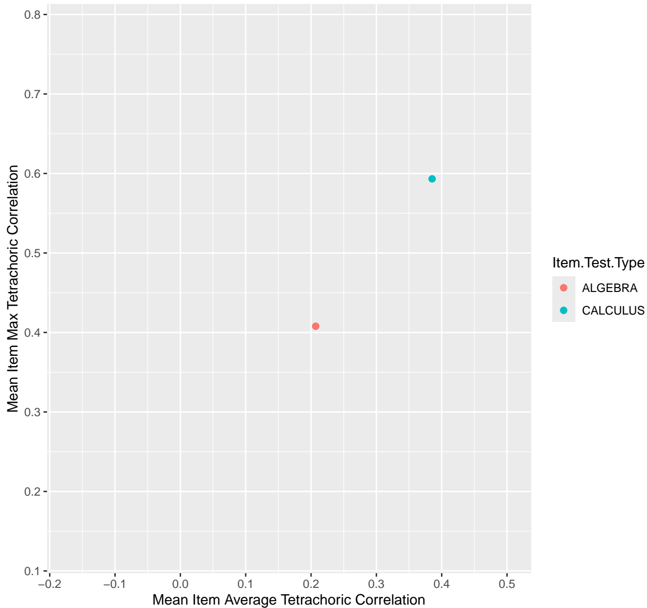
Mean Item Average vs Max Tetrachoric Correlation For KD1.38.V3AH
