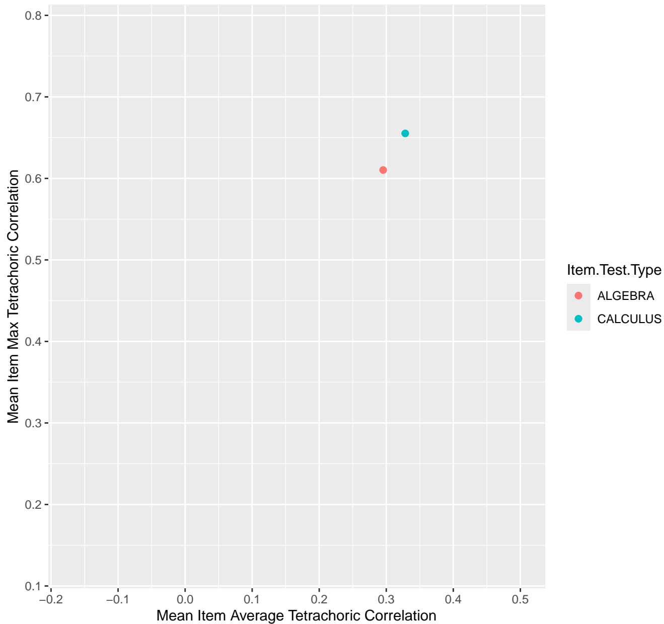
Mean Item Average vs Max Tetrachoric Correlation For KD1.20.V1
