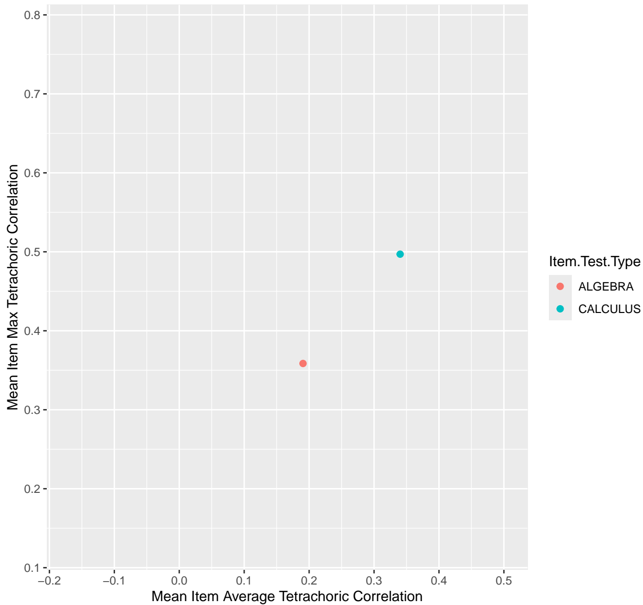
Mean Item Average vs Max Tetrachoric Correlation For KD1.35.V3AH
