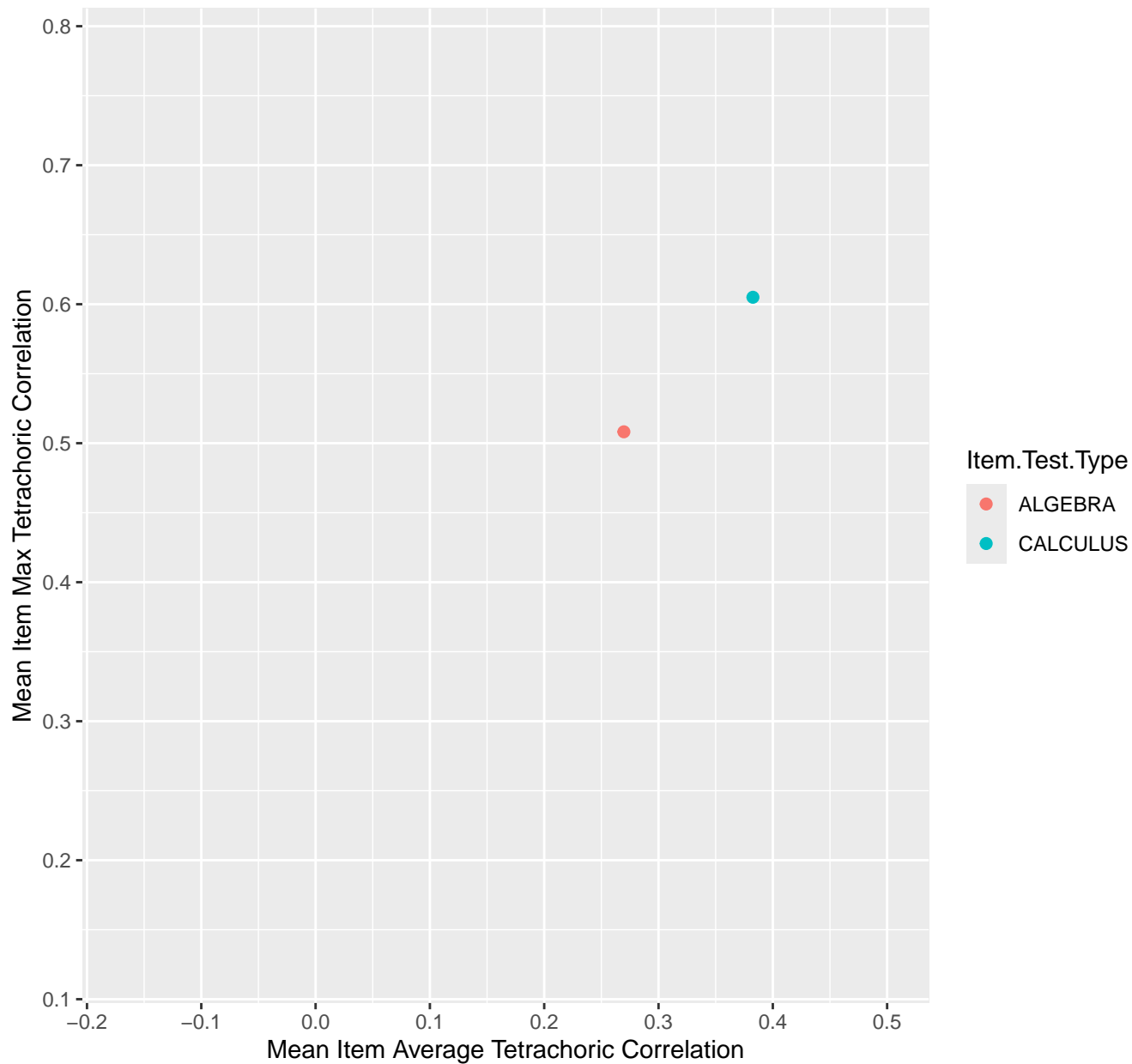
Mean Item Average vs Max Tetrachoric Correlation For KD1.35.V1
