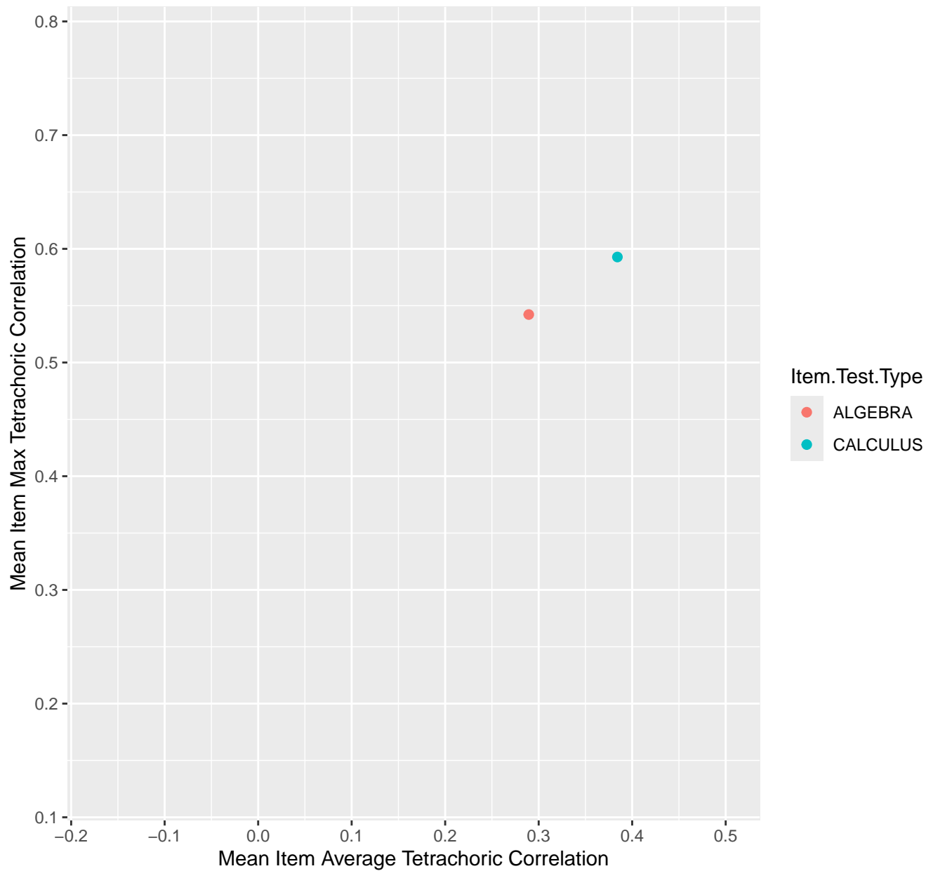
Mean Item Average vs Max Tetrachoric Correlation For KD1.38.V1
