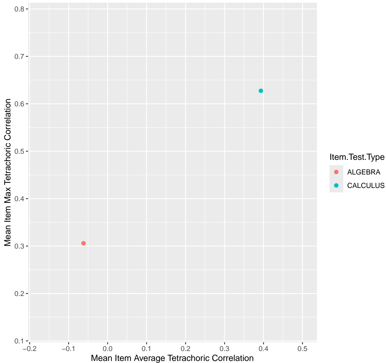
Mean Item Average vs Max Tetrachoric Correlation For KD1.28.V1
