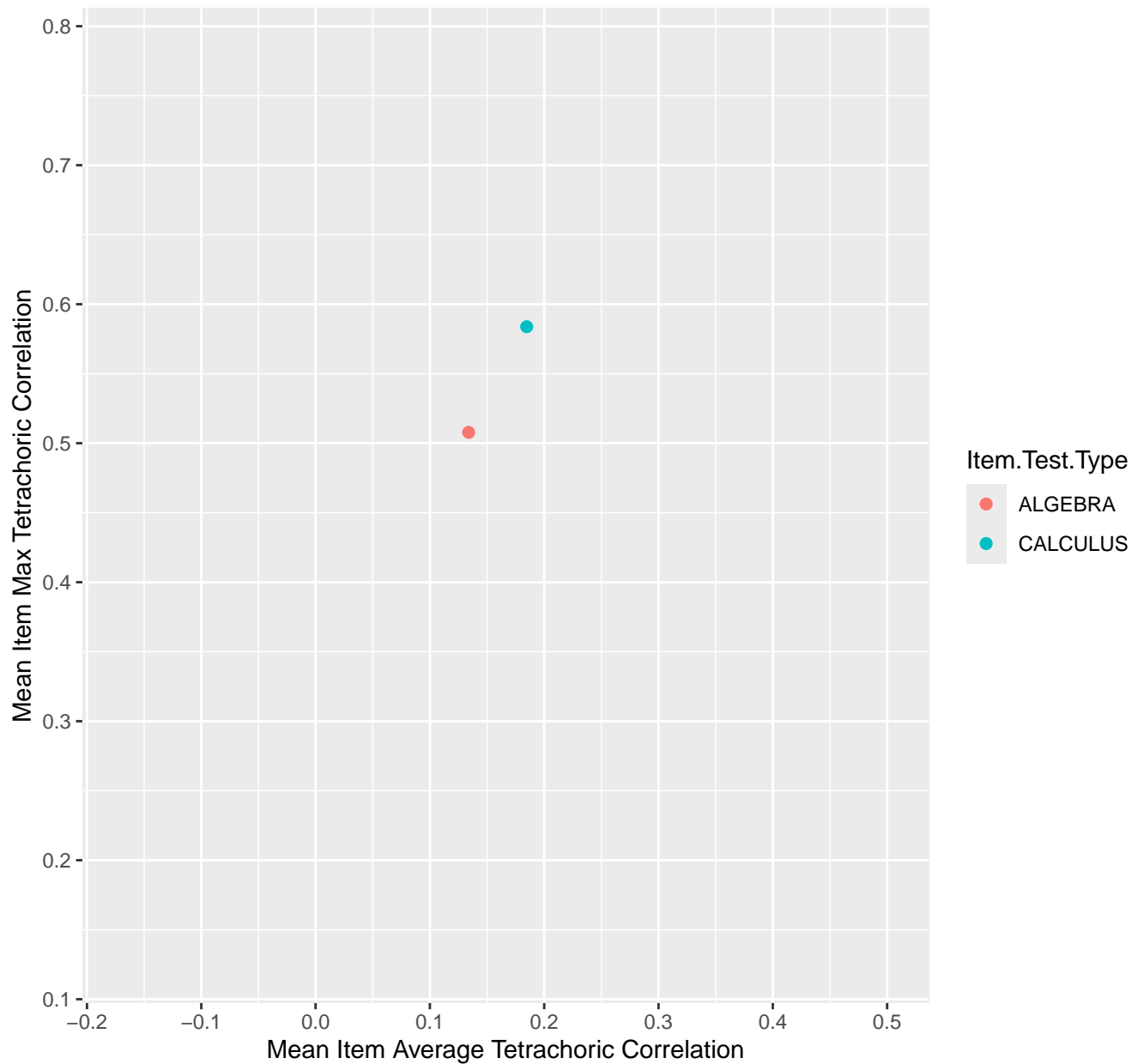
Mean Item Average vs Max Tetrachoric Correlation For KD1.1.V1
