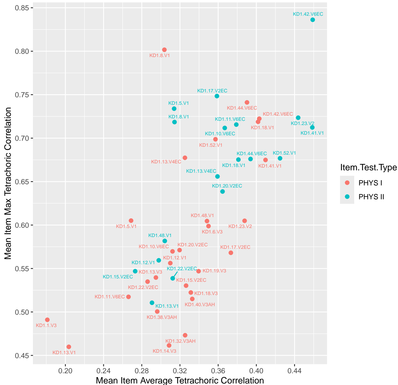
Mean Item Average vs Max Tetrachoric Correlation
